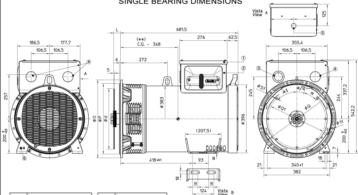
SINGLE BEARING DIMENSIONS
